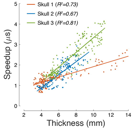
Figure 7: Ultrasound phase distortion is proportional to skull thickness. Ultrasound speedup through individual segments of the skull as a function of skull thickness. The R^2 values listed in the inset provide the amount of variance explained by the linear fits superimposed on the plots.
