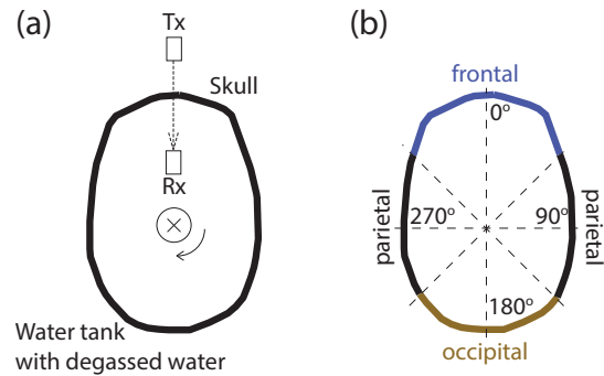
Figure 1: Through-transmit measurements across intact skulls.
