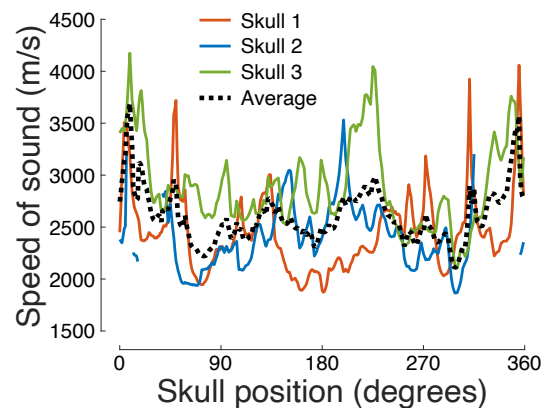
Figure 8: Speed of sound across the skull. The speed of sound ( c_s ) determined from the through-transmit \tau values (see Materials and Methods) as a function of the skull position.
